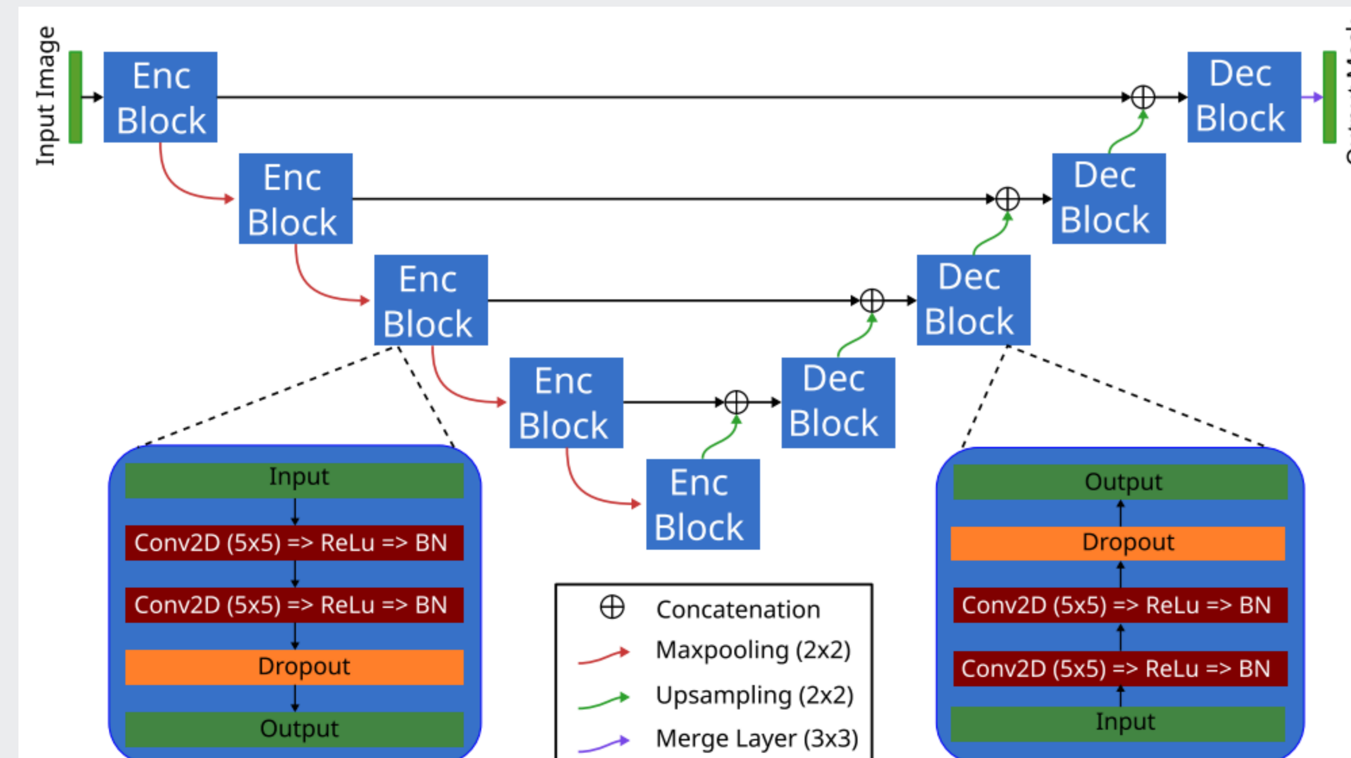
Figure 3: Probabilistic Bayesian U-Net architecture. Taken from [4].
