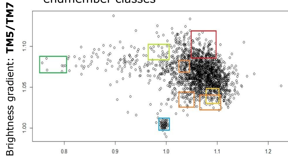
Fig. 8: scatterplot of TM5/TM4 and TM5/TM7 bands with the position of the endmember classes
