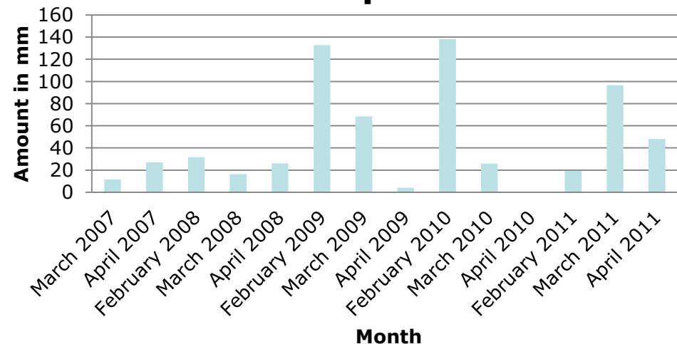
Fig. 18: Precipitation levels for the period during and before the satellite overflight
