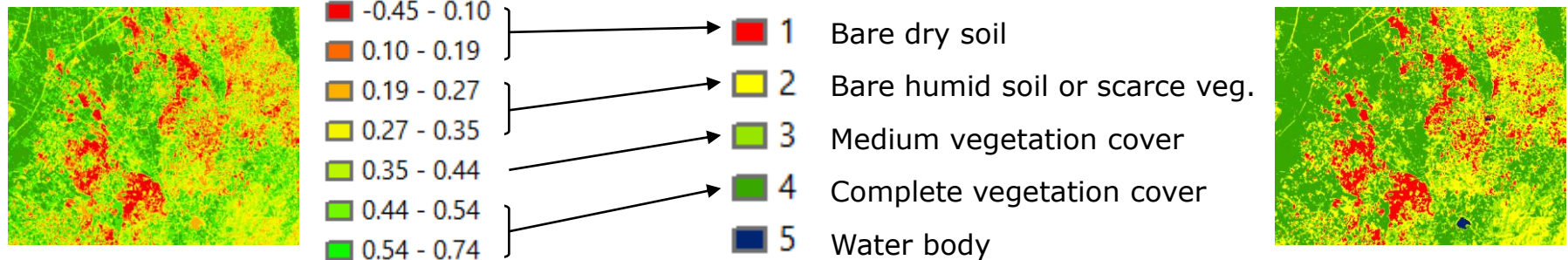
Fig. 5: initially 7 classes reclassified into 5
