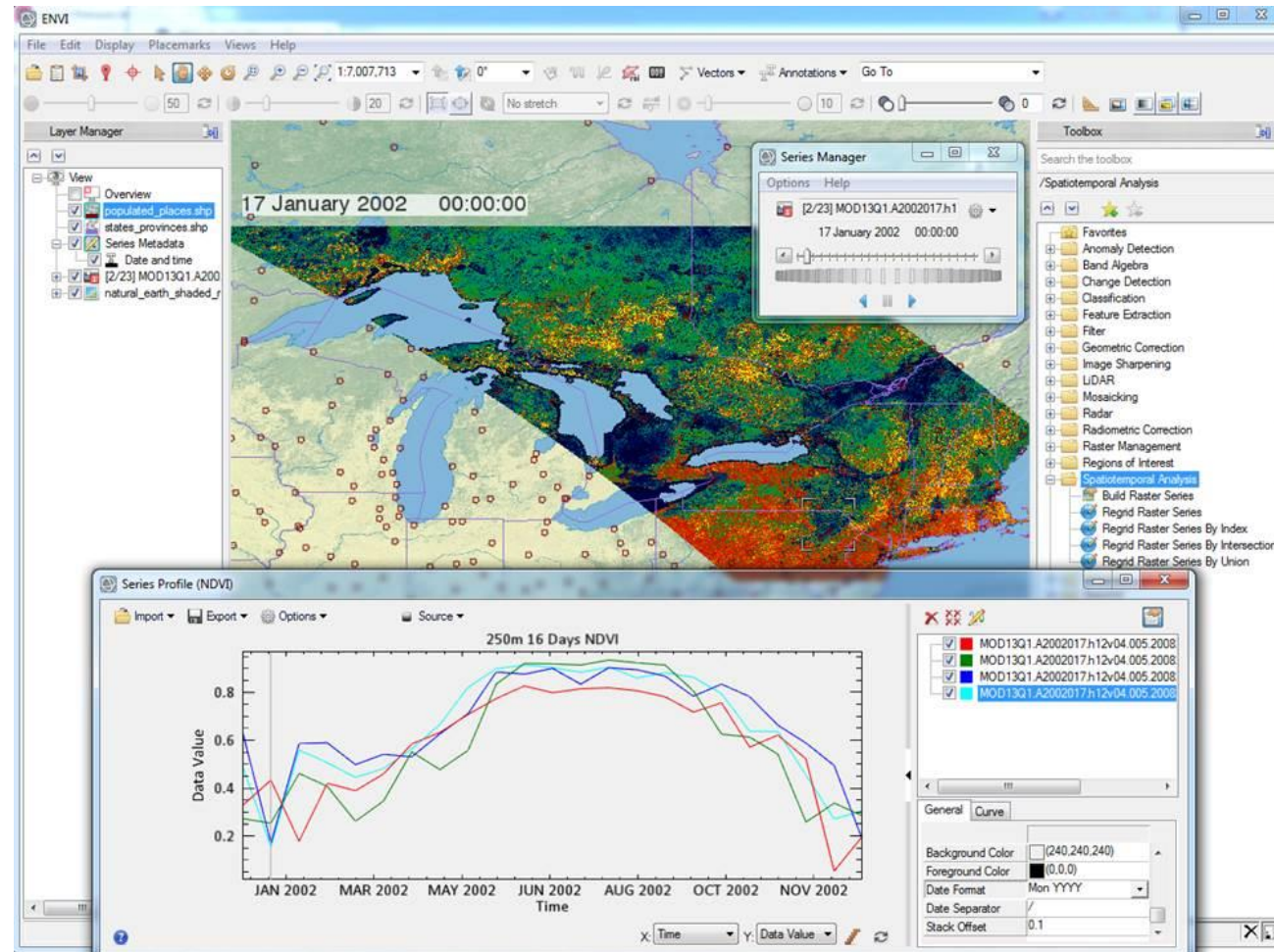
Temporal NDVI analysis using MODIS
